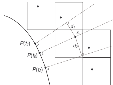
Figure 19: Computation of foot-points on a fitting curve.
