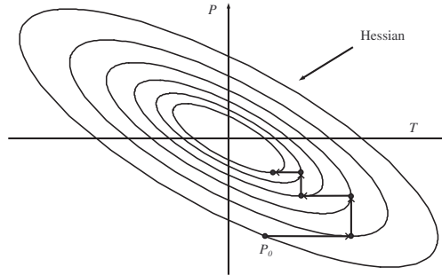
Figure 24: The alternating minimization steps of PDM. \mathcal{P} and \mathcal{T} stand for the linear subspaces spanned by the control points P_i and the data parameters t_k .
