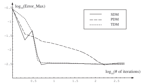
Figure 8: (Example 1) Comparison of the three methods on sparse data points a circle (Number of data points: 32). Log scale (base 10) is used for the error axis. In this figure the iteration axes in Figures (e) and (f) use log scale (base 10) in order to distinguish the error curves of TDM and SDM.
